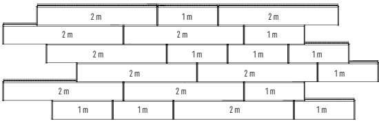
ASSEMBLY WITH Z-301 CONNECTOR
