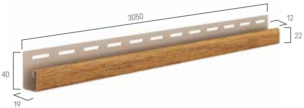
SVP(U)-15 Connector
